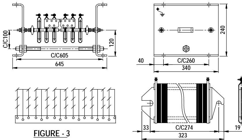
RESISTANCE BOX TYPE FGR-1111
